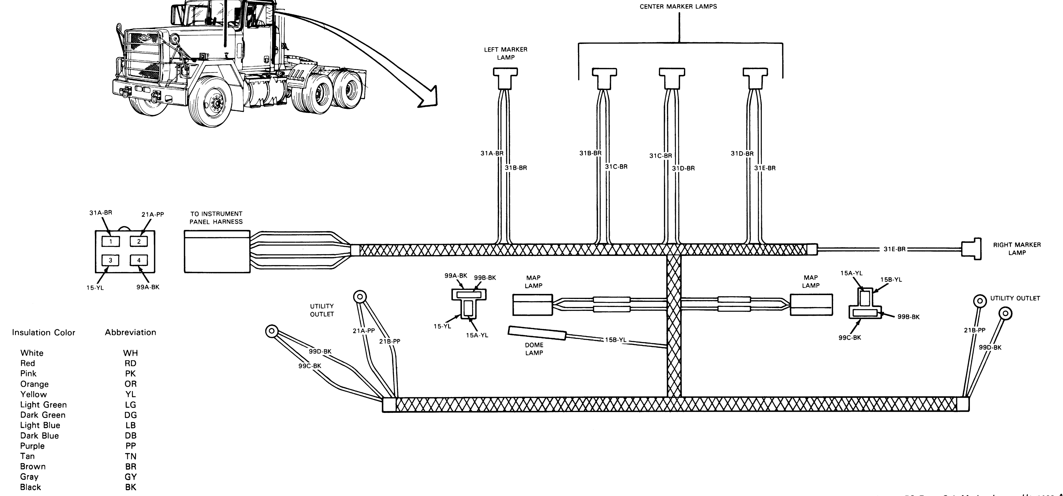
Figure FO-7. Cab Marker Lamps Harness Assembly
