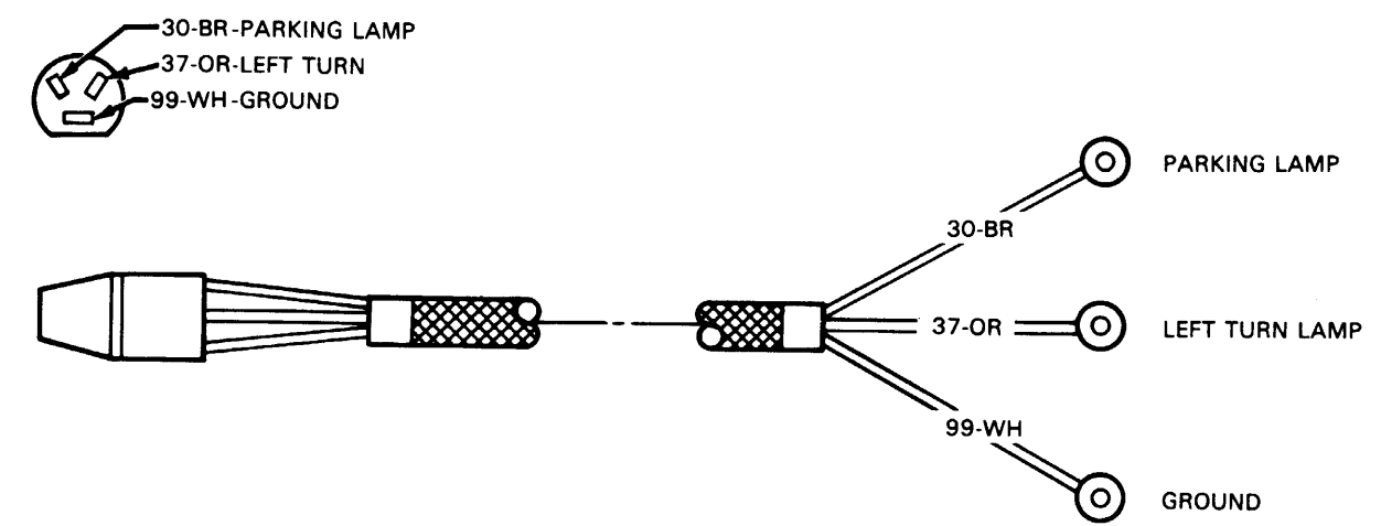
LEFT HAND HARNESS
