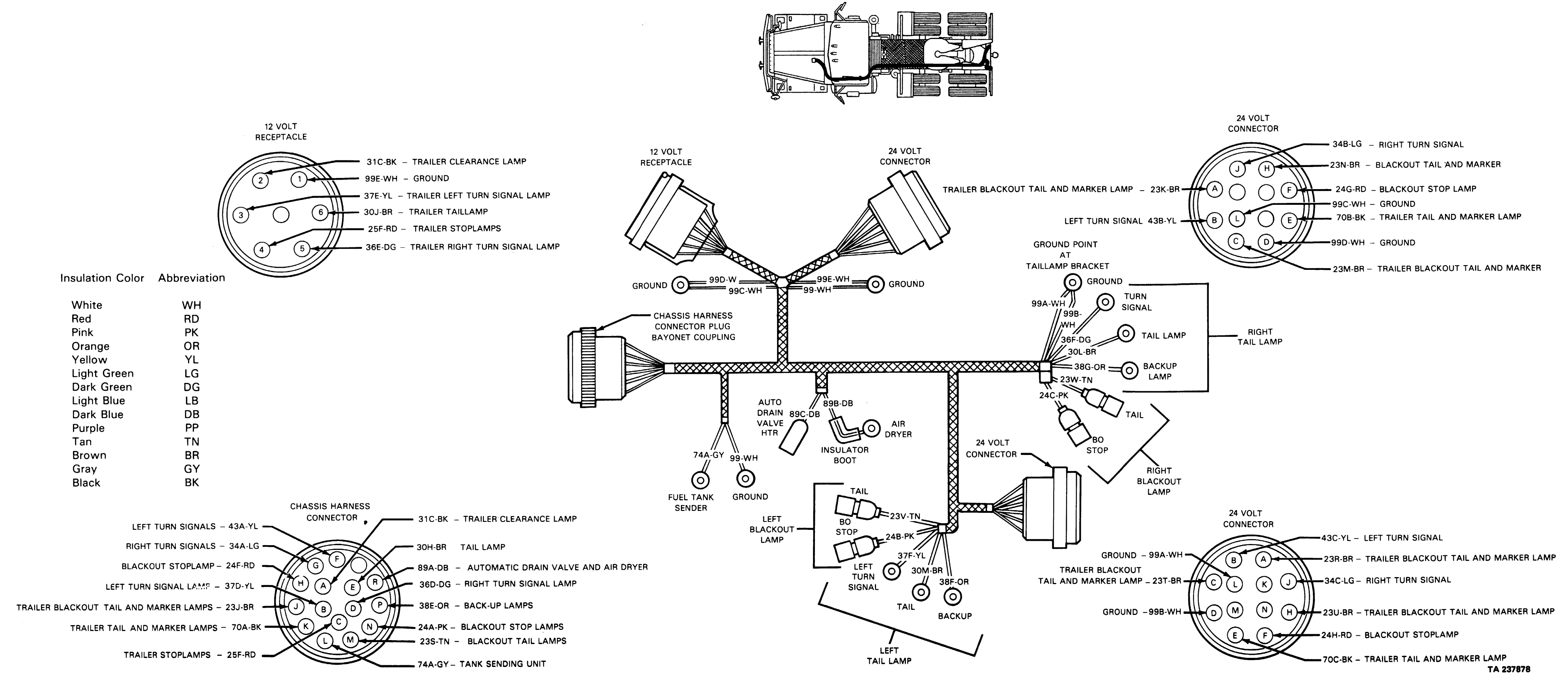
Figure FO-11. Chassis Harness Assembly FO-11 (FO-12 BLANK)
